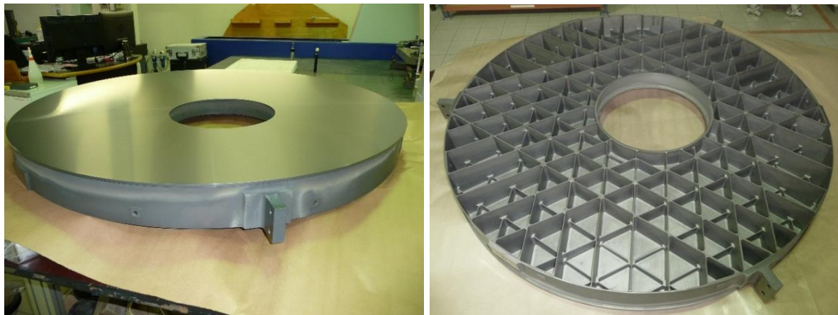
Fig. 7. The ready-to-polish M1 blank Flight Model, front face (left picture) and rear face (right)
