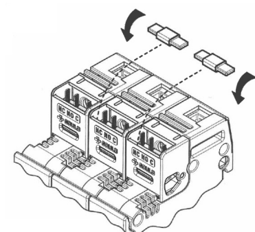
Assemblés 3 x CMS14W1 + 2 X CMS1422PTH
