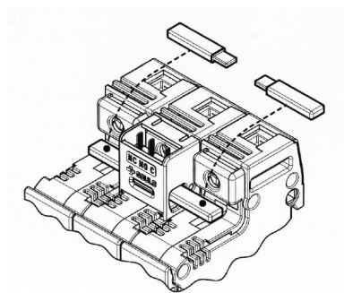
CMS14W1 + CMS1422BP
